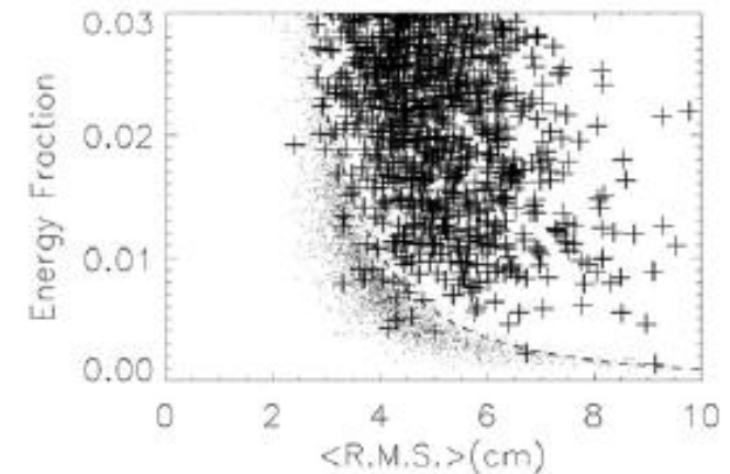
Fig. 4: Separation of electrons (dot) and protons (cross)
