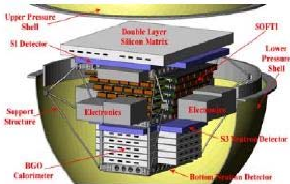
Fig. 1: Diagram of the ECAL concept payload
